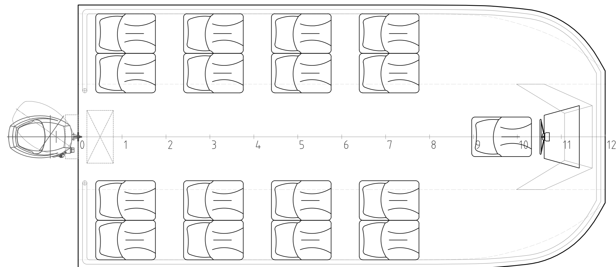
DECK PLAN SCALE 1:25
