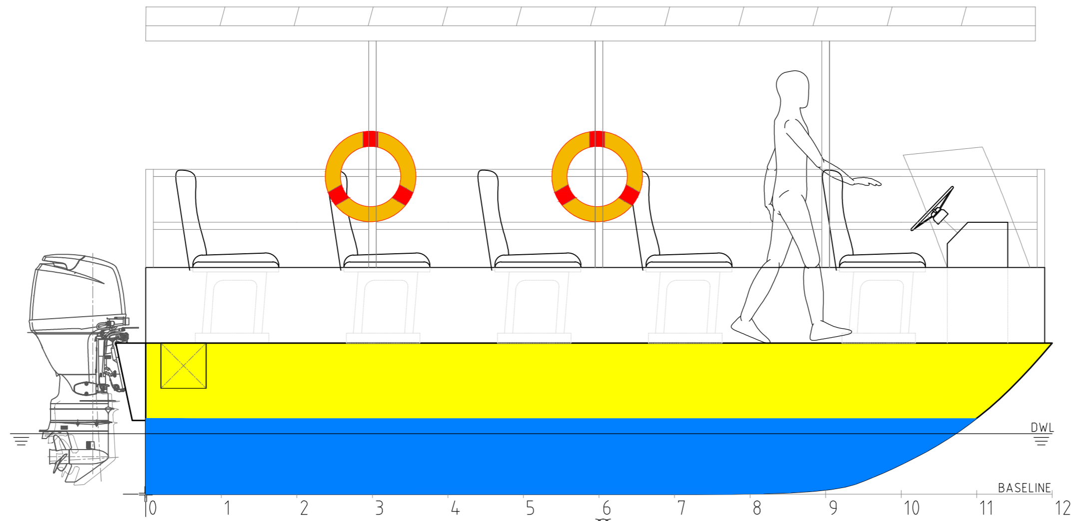
PROFILE SCALE 1:25
